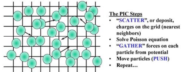
Figure 9. Particles in cell (PIC) steps [ES05]
